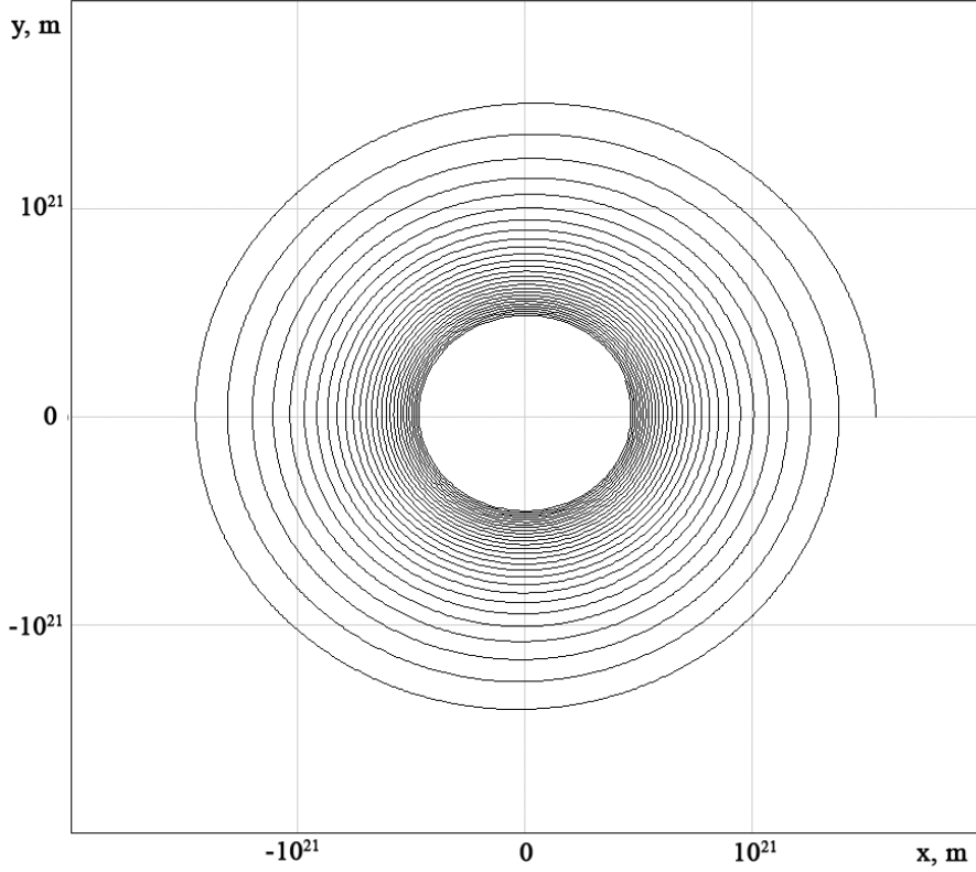
Figure 3: A star orbit in a galaxy with M = 10^{10} \cdot M_{\odot} by u = 5 \cdot 10^5 m/s and r(0) = 100 kpc for the case of w = 10^{-4} \cdot H_0 c ; t = 300 Gyr, the first unclosed external loop corresponds to 27.6 Gyr.
