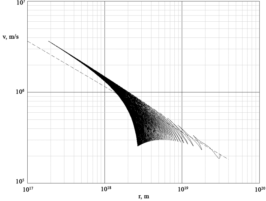
Figure 2: The graph of v(r) for the star orbit in a galaxy with M = 10^{10} \cdot M_{\odot} by u = 5 \cdot 10^5 m/s and r(0) = 1 kpc (solid line). For comparison, the graph of v_0(r) \equiv (G \cdot M/r)^{0.5} is shown (dashed line).
