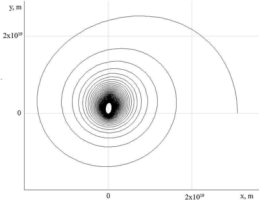
Figure 1: A star orbit in a galaxy with M = 10^{10} \cdot M_{\odot} by u = 5 \cdot 10^5 m/s and r(0) = 1 kpc.
